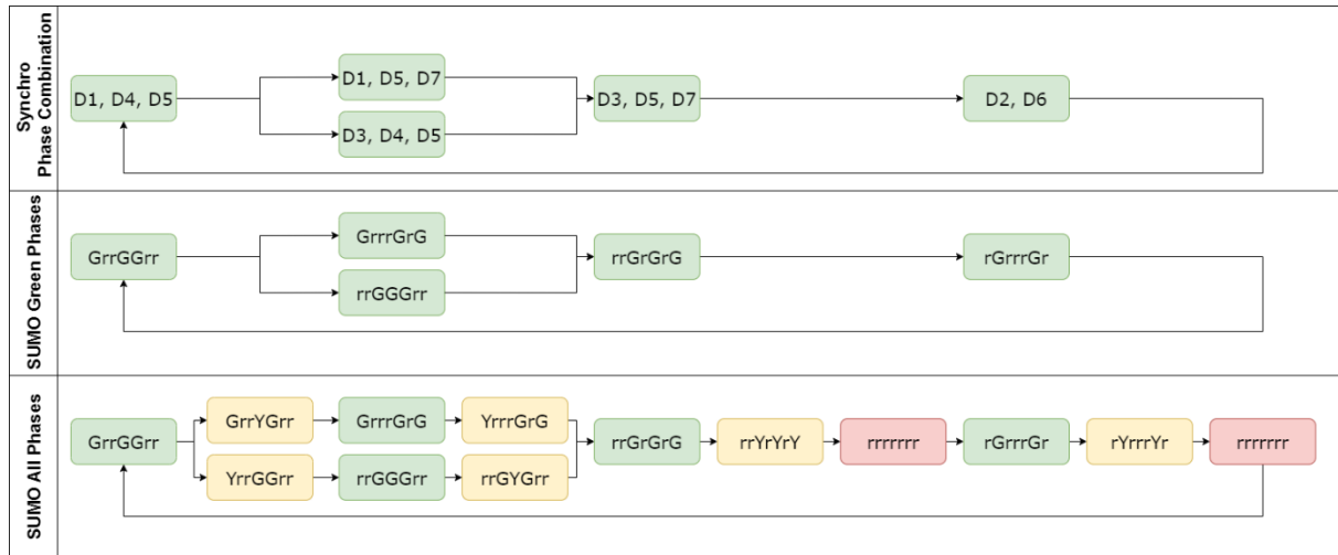
Figure 10. Signal Phase Mapping Example
