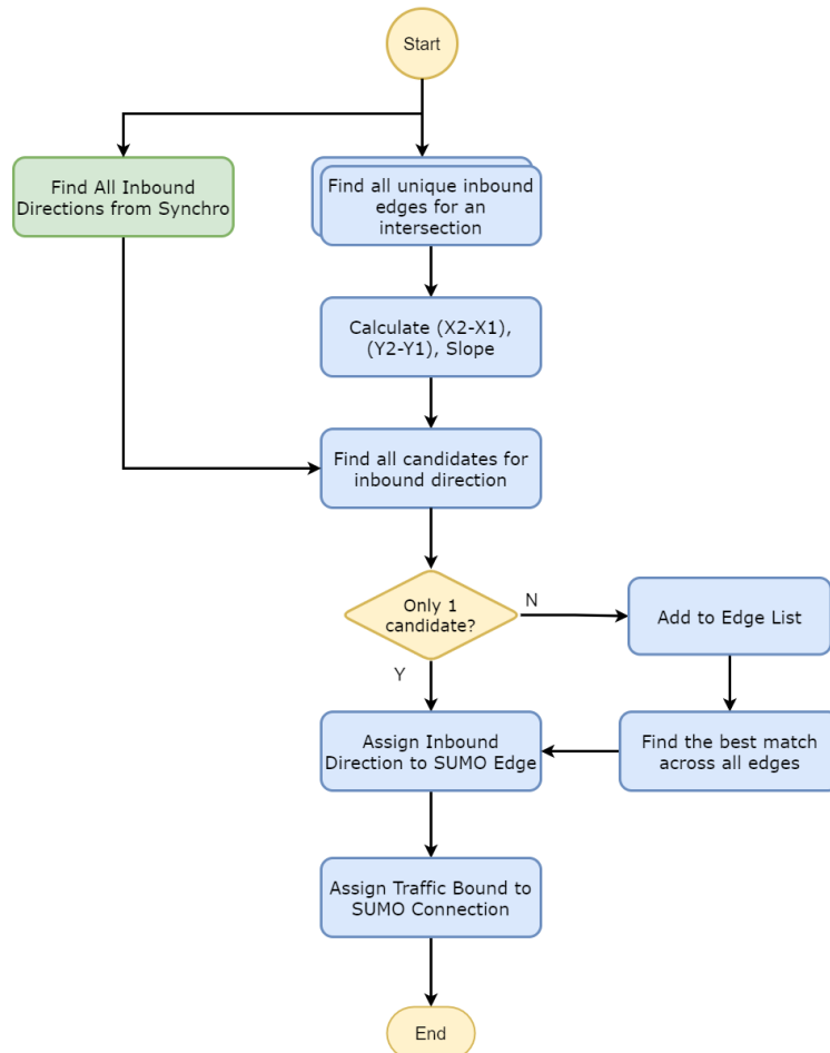
Figure 8. SUMO connection to Synchro direction mapping process
